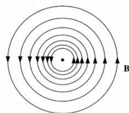
(b) Magnetostatic field of a long wire
