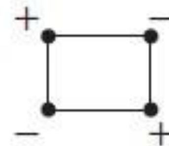
Quadrupole ( V \sim 1/r^3 )
