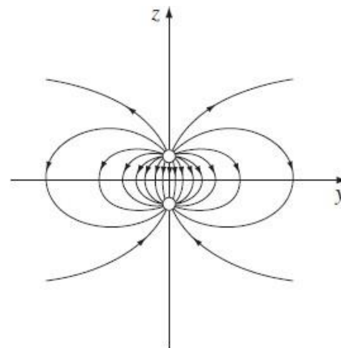
(b) Field of a "physical" dipole
