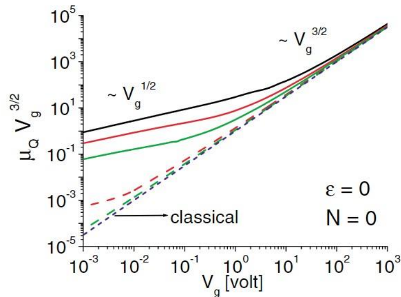
FIG. 2 (color online). The values of \mu_Q V_g^{3/2} as a function of gap voltage V_g (volt) for various gap spacing D = 1, 10, \text{ and } 100 \text{ nm} (solid lines: top to bottom). The dashed lines are without an exchange-correlation term ( \phi_{xc} = 0 ) for D = 10 and 100 \text{ nm} (top to bottom), and the short-dashed line is the classical limit.
