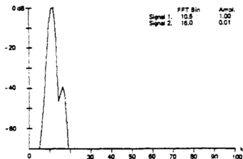
Fig. 64. \text{Cos}^4(\pi\pi/N) window.
