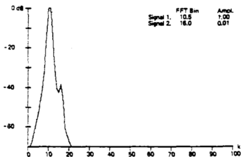
Fig. 62. \text{Cos}^2(\pi\pi/N) window.
