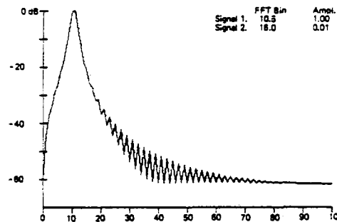
Fig. 80. Poisson window ( \alpha = 4.0 ).
