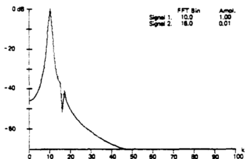
Fig. 61. \text{Cos}(\pi\pi/N) window.
