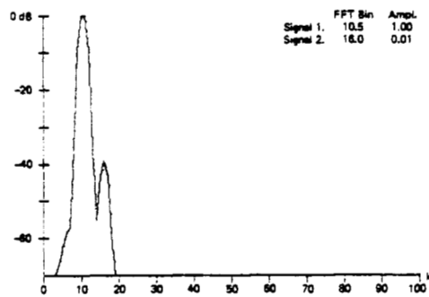
Fig. 66. Blackman window.
