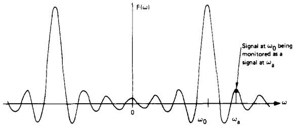
Fig. 10. Spectral leakage effect of window.
