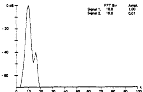
Fig. 63. \text{Cos}^3(\pi\pi/N) window.
